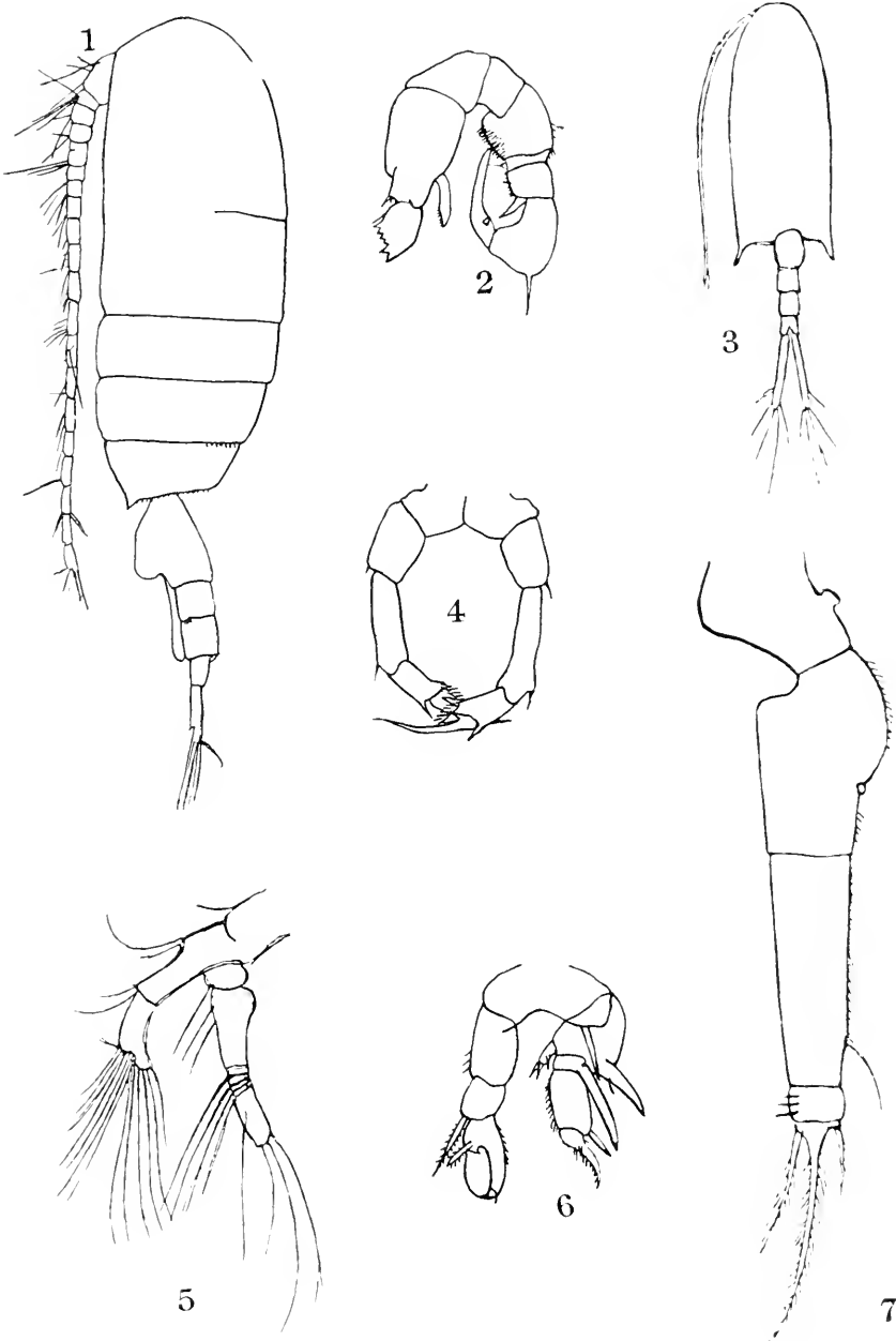
1, 2, 4 Pseudodiaptomus acutus : 1, Whole animal; 2, Fifth feet of male; 4, Fifth feet of female. (After Dahl, 1894.) 3, 5-7. Pseudodiaptomus aurivilli : 3, Whole animal (after Cleve, 1901); 5, second antenna (after Cleve, 1901); 6, fifth feet of female (after Thompson and Scott, 1903); 7, fifth feet of female (after Thompson and Scott, 1903).
